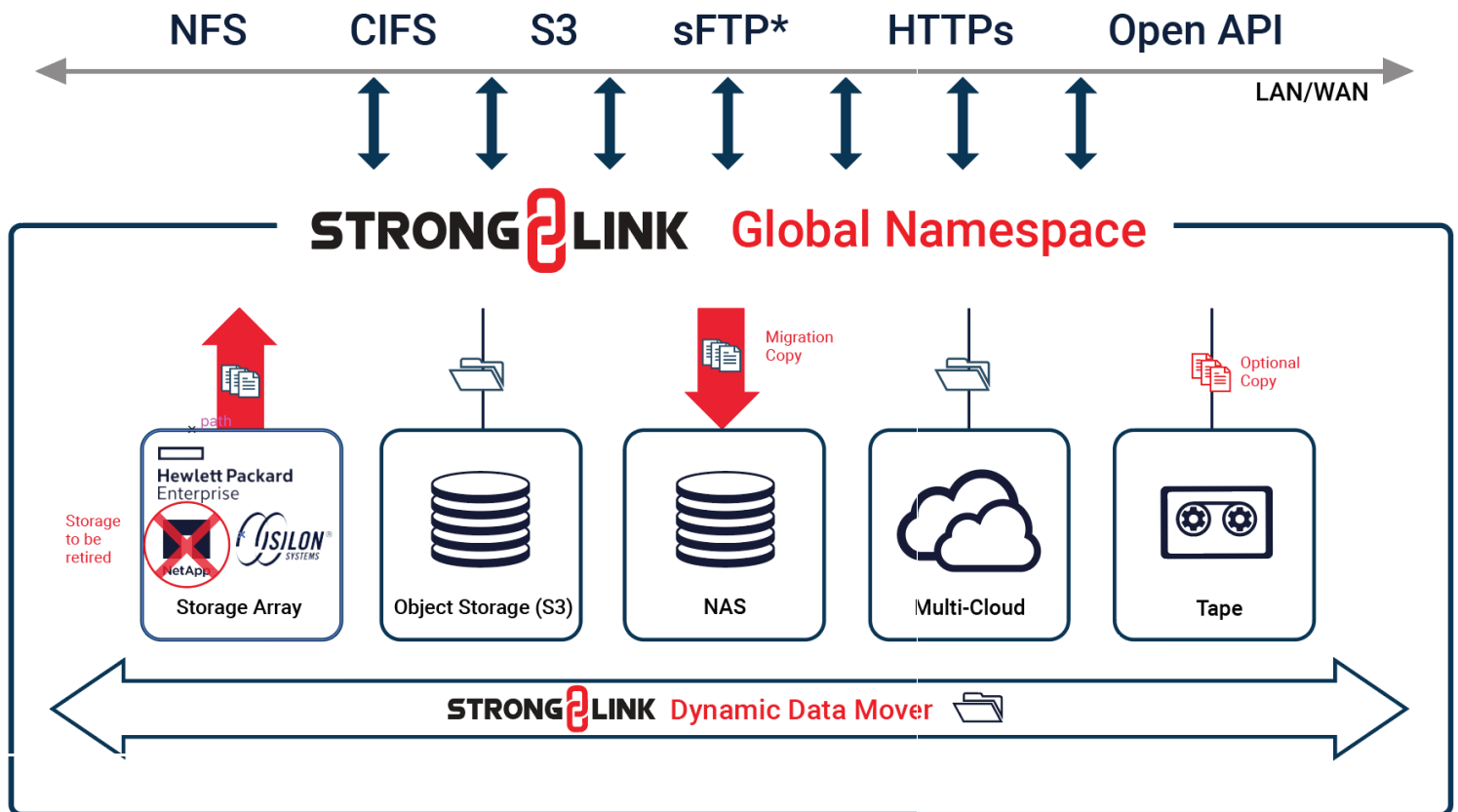
Figure 1. StrongLink ensures copies are migrated from the source storage to new target storage and verified
